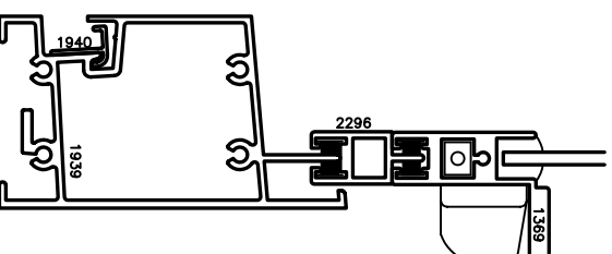
④ STANDARD SILL
