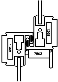
OPTIONAL 1368 MEETING RAIL (FOR LARGE WINDOWS REQUIRING 60 PSF STRUCTURAL LOAD)
