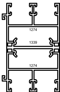
#1339 MULLION
