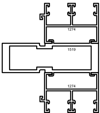
#1519 MULLION
