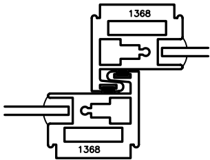
OPTIONAL 1368 MEETING RAIL (FOR LARGE SASH REQUIRING 90 PSF STRUCTURAL LOAD)
