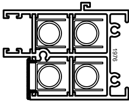
OPTIONAL HEAD BALANCE TOP & BOTTOM SASH
