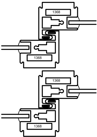
1368 MEETING RAILS (FOR LARGE WINDOWS REQUIRING 90 PSF STRUCTURAL LOAD)
