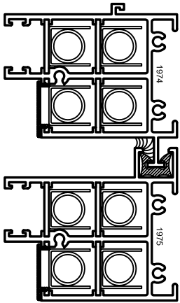
HEAD BALANCE TOP & BOTTOM SASH
